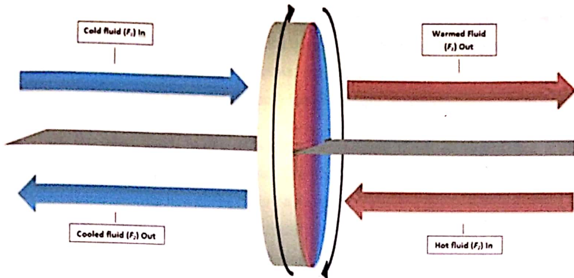
Figure 9 Heat Transfer In A Rotary-Type Regenerator
