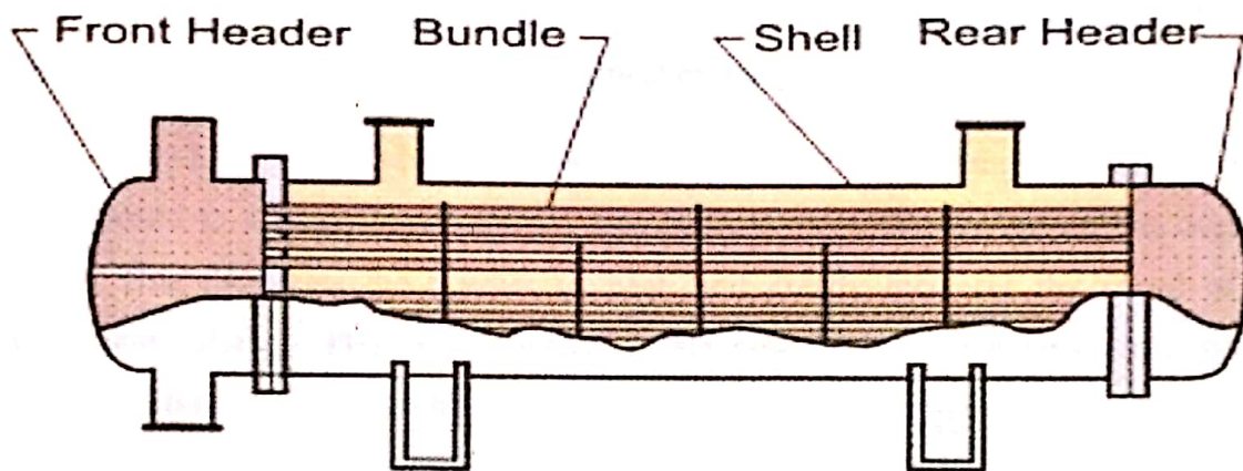
Figure 4 Shell And Tube Heat Exchanger
