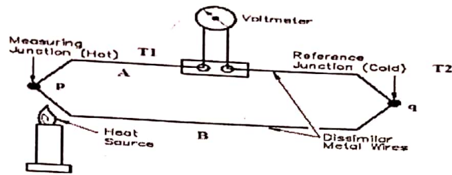
Thermocouple Circuit
