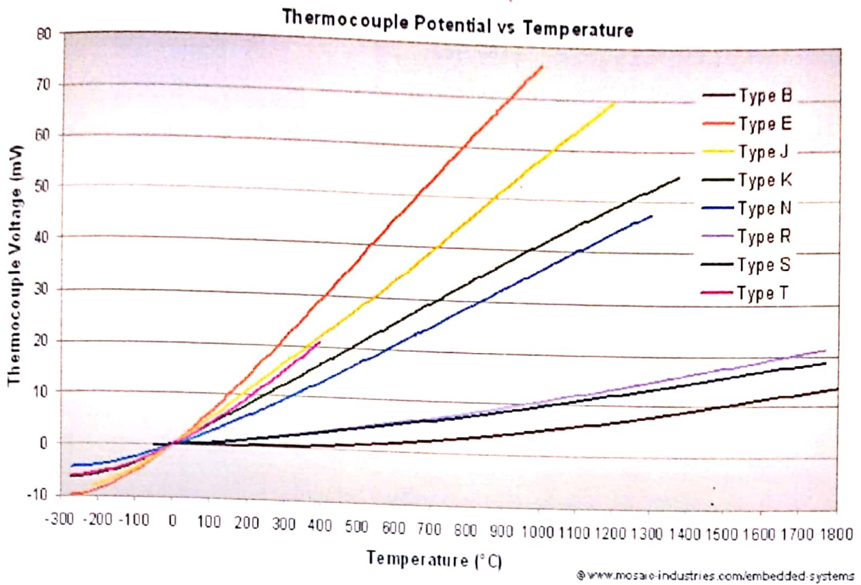
Figure 11 Thermocouple potential vs Temperature plot
