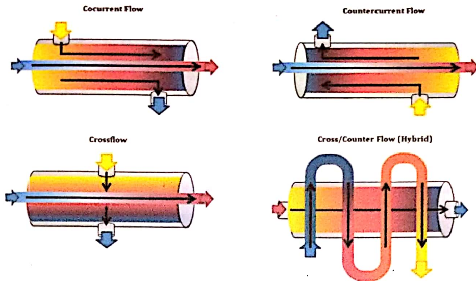
Figure 2 Types Of Heat Transfer In Heat Exchangers
