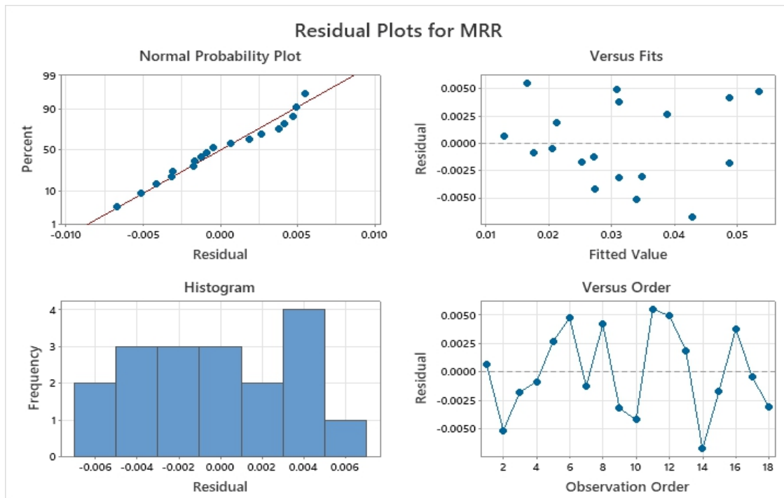
Figure 5.2: Residual plots for MRR
