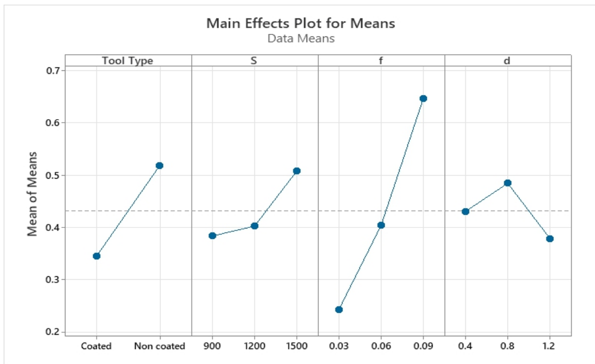
Figure 5.3 : Main Effects Plots for Means of Ra
