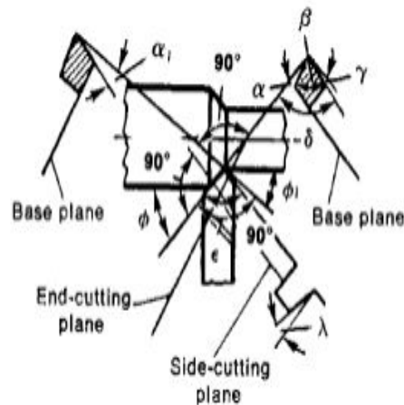
Fig. 1.3 Cutting Angles
