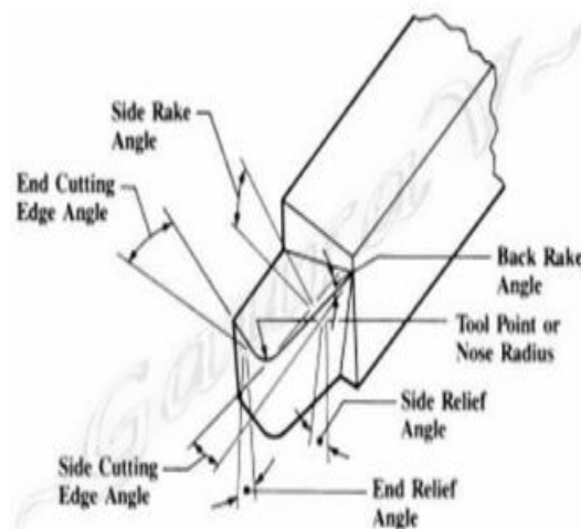
Figure. 1.4 Tool Geometry
