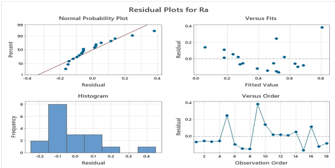
Figure 5.4 :Residual plots for Ra
