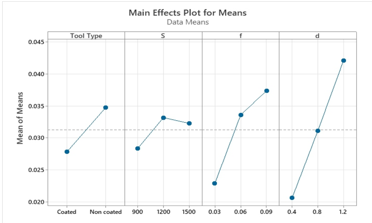
Figure 5.1 Main Effects Plots For Means of MRR
